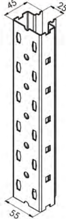
55A Upright
