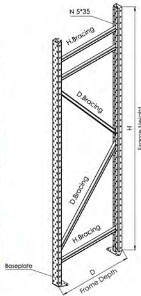
2 Uprights Frame
