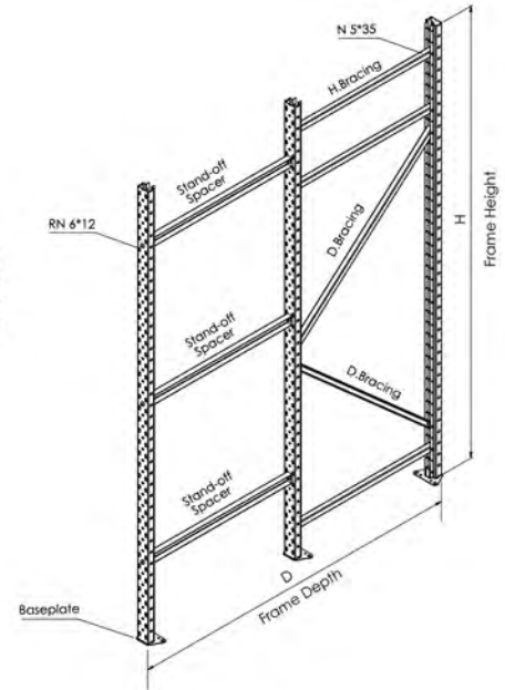
3 Uprights Frame
